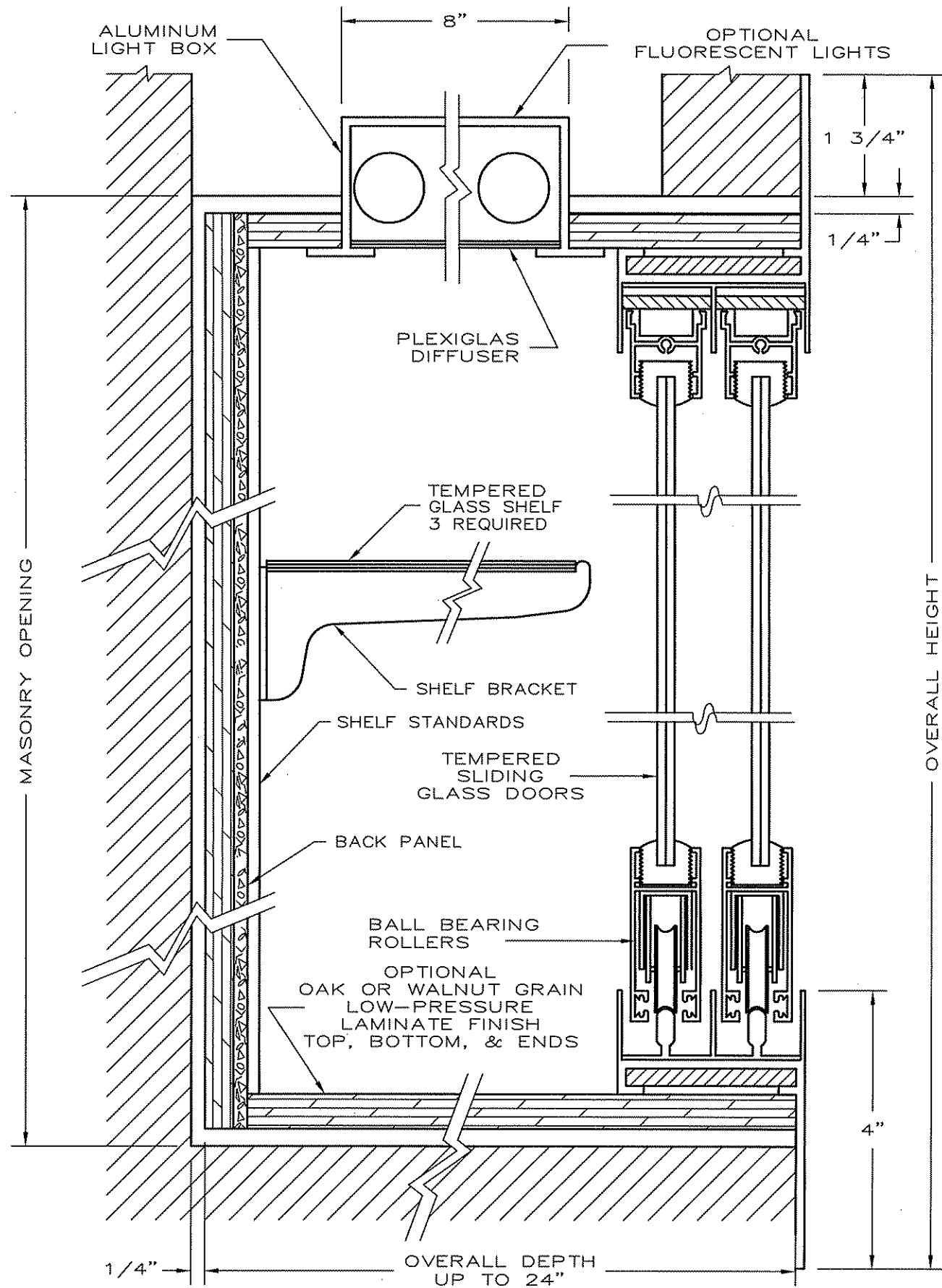
SECTION "AA"
