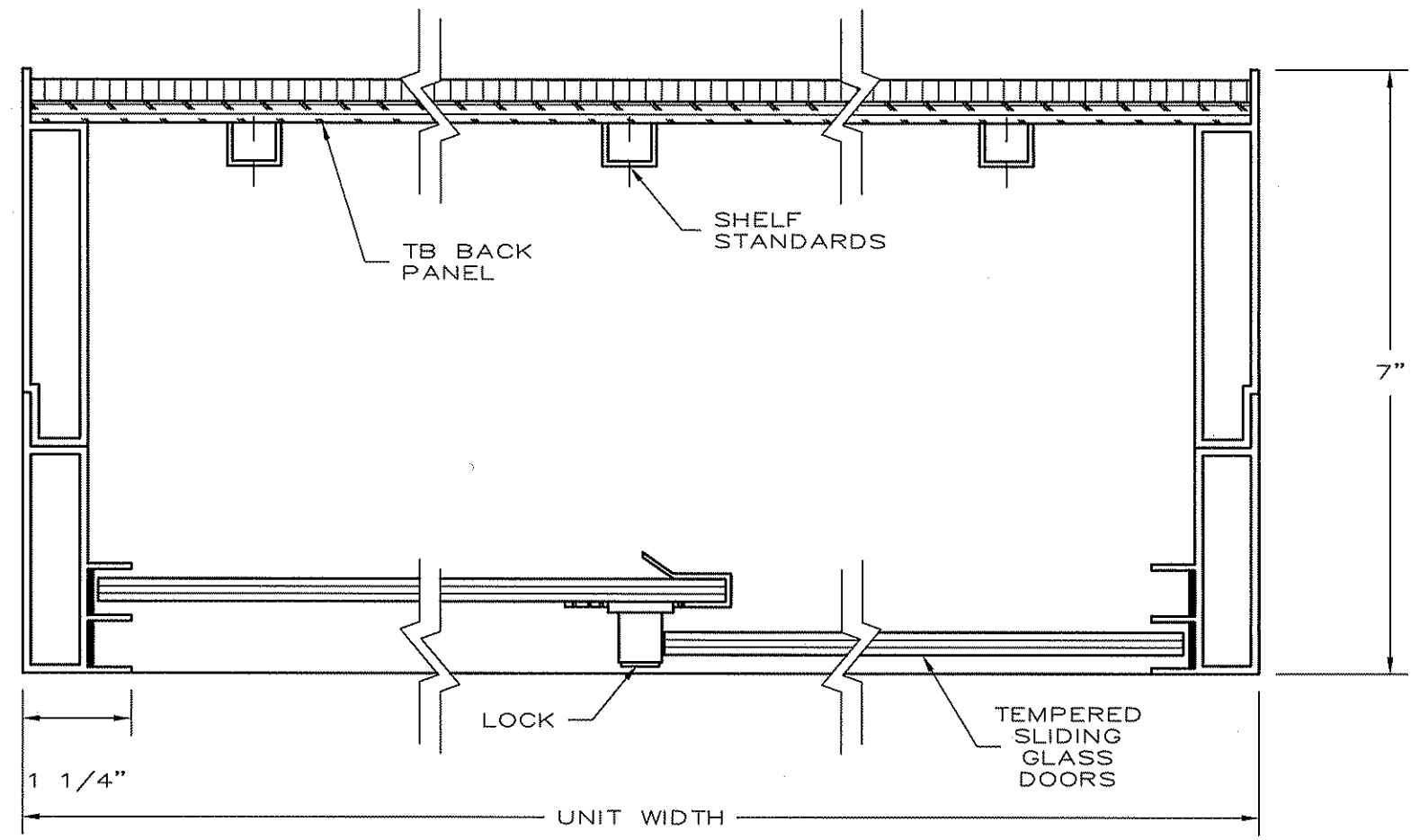
SECTION "B"
