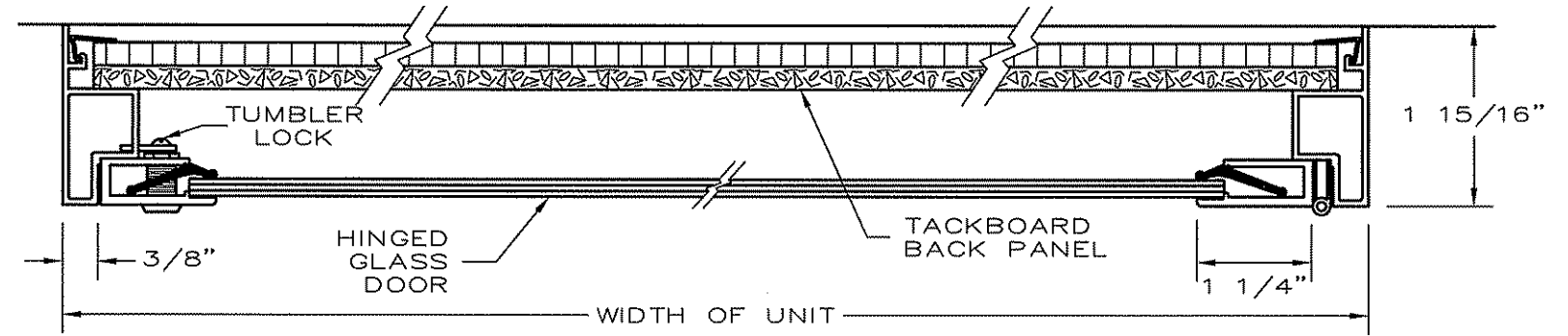
SECTION "B"
